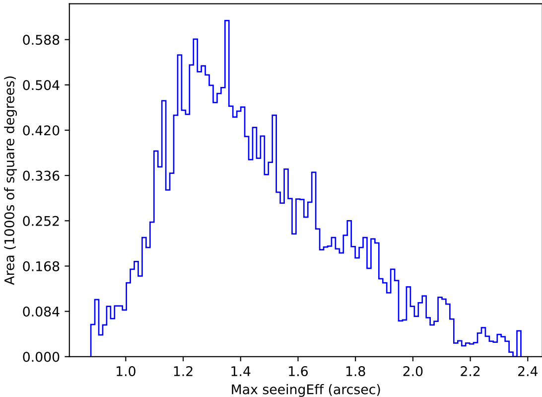
baseline_v2.0_10yrs Yr 1 u band: Max seeingEff
