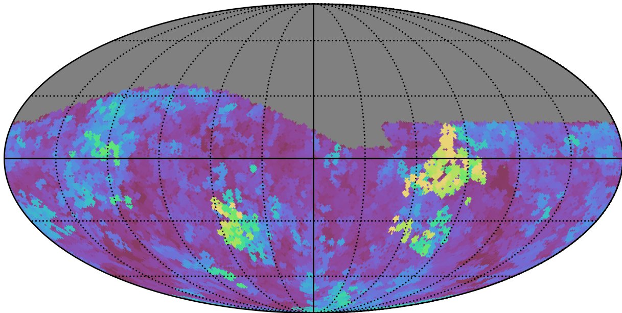
baseline_v2.0_10yrs Yr 1 r band: Max seeingEff
