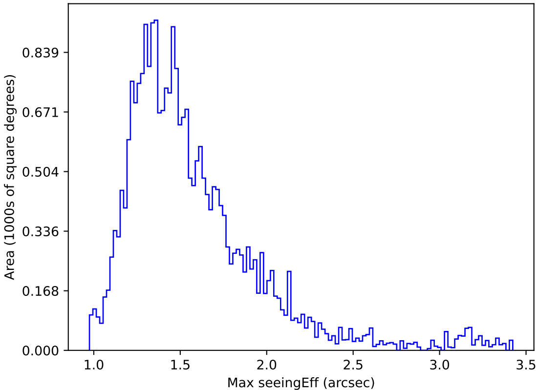
baseline_v2.0_10yrs Yr 1 r band: Max seeingEff
