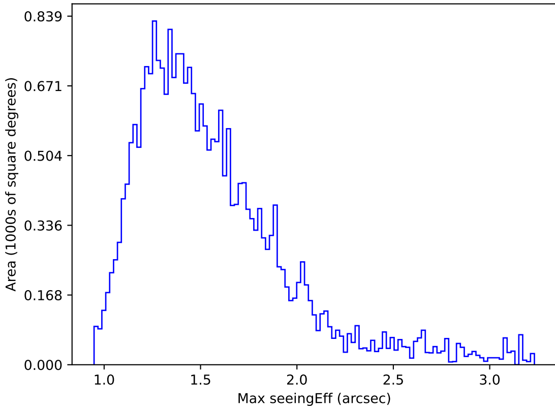
baseline_v2.0_10yrs Yr 1 i band: Max seeingEff
