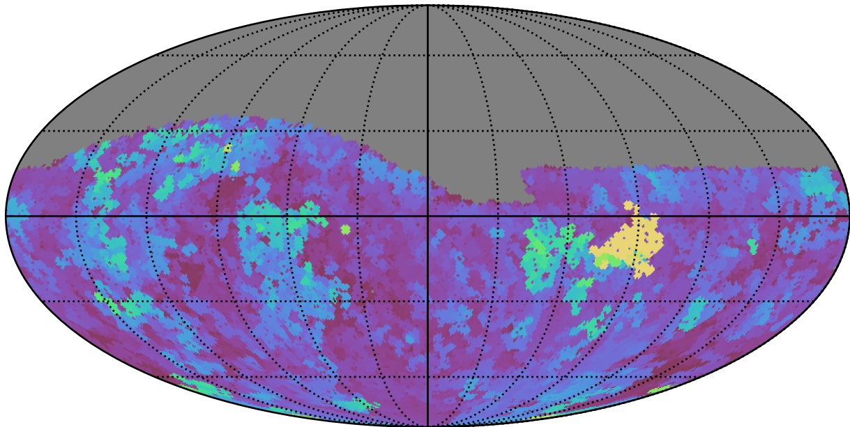
baseline_v2.0_10yrs Yr 1 g band: Max seeingEff
