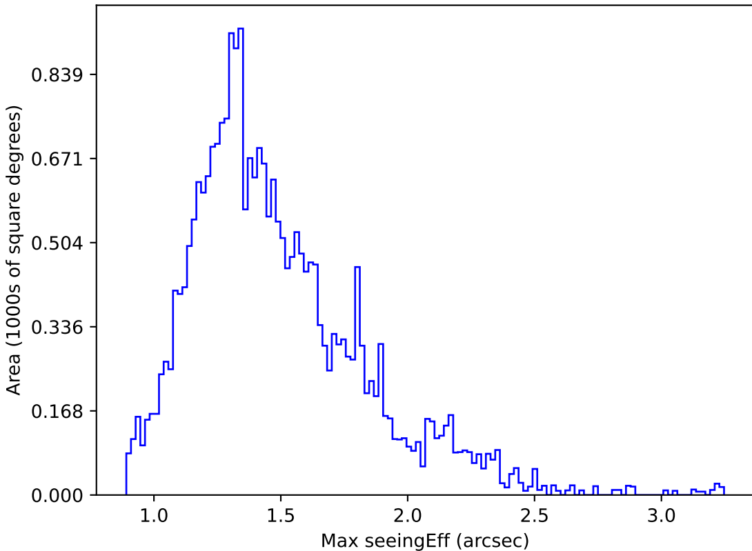
baseline_v2.0_10yrs Yr 1 g band: Max seeingEff
