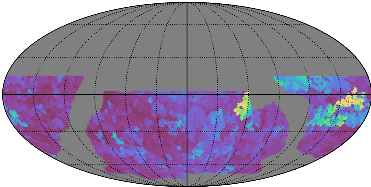
baseline_v2.0_10yrs WFD y band: Max seeingEff
