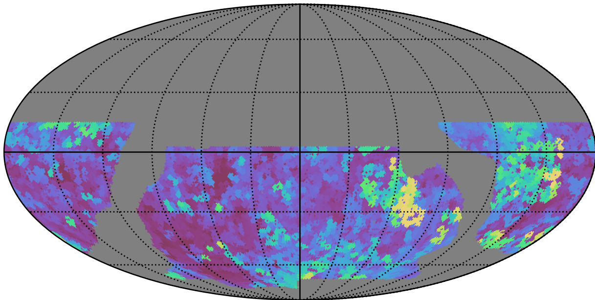
baseline_v2.0_10yrs WFD u band: Max seeingEff
