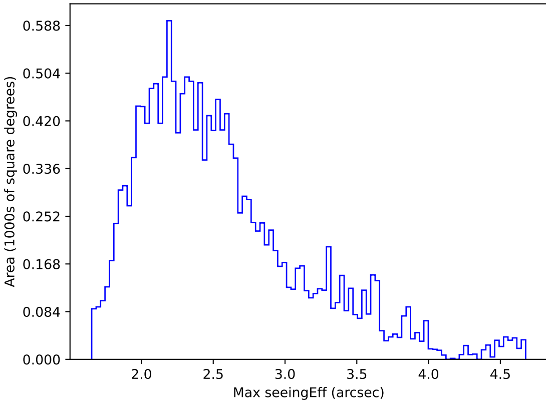
baseline_v2.0_10yrs WFD u band: Max seeingEff
