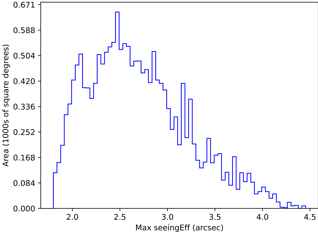
baseline_v2.0_10yrs WFD r band: Max seeingEff
