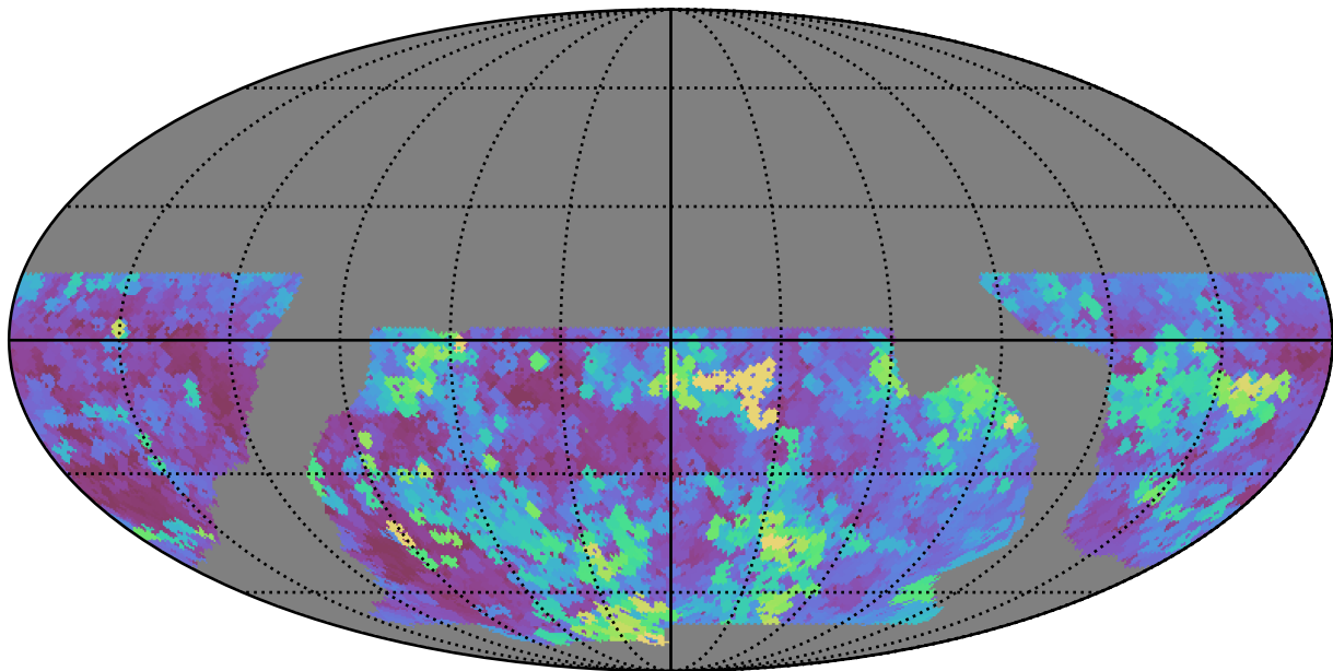
baseline_v2.0_10yrs WFD g band: Max seeingEff
