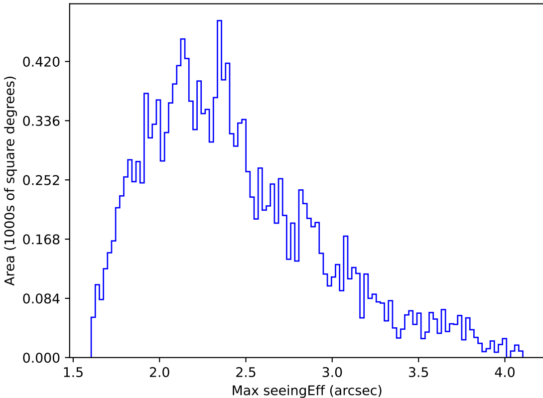
baseline_v2.0_10yrs WFD g band: Max seeingEff
