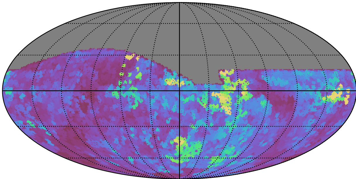
baseline_v2.0_10yrs All sky z band: Max seeingEff
