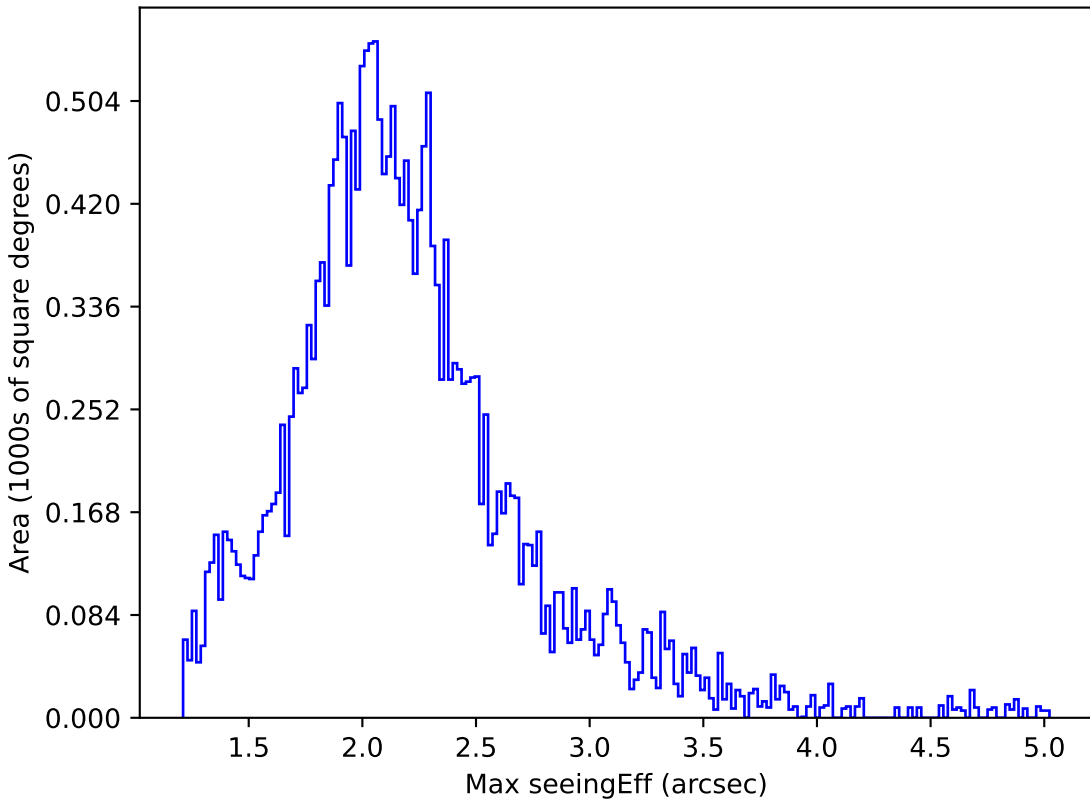
baseline_v2.0_10yrs All sky y band: Max seeingEff
