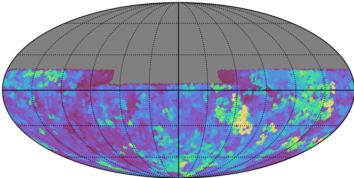
baseline_v2.0_10yrs All sky u band: Max seeingEff
