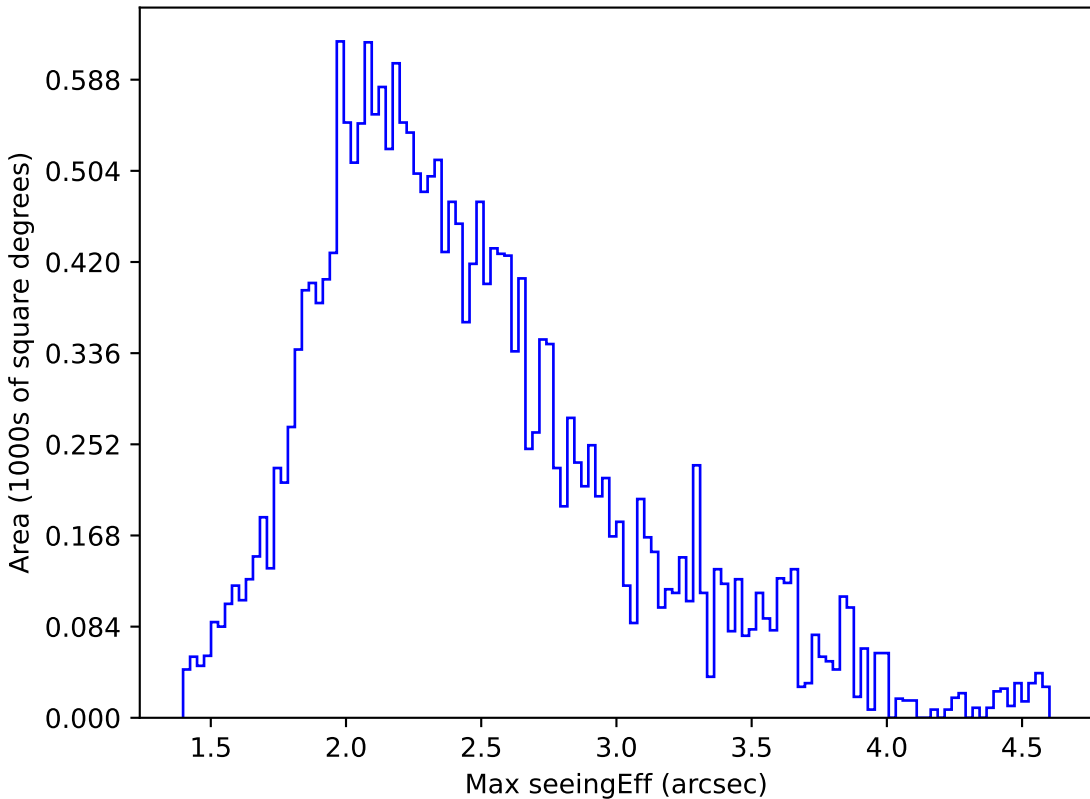
baseline_v2.0_10yrs All sky u band: Max seeingEff
