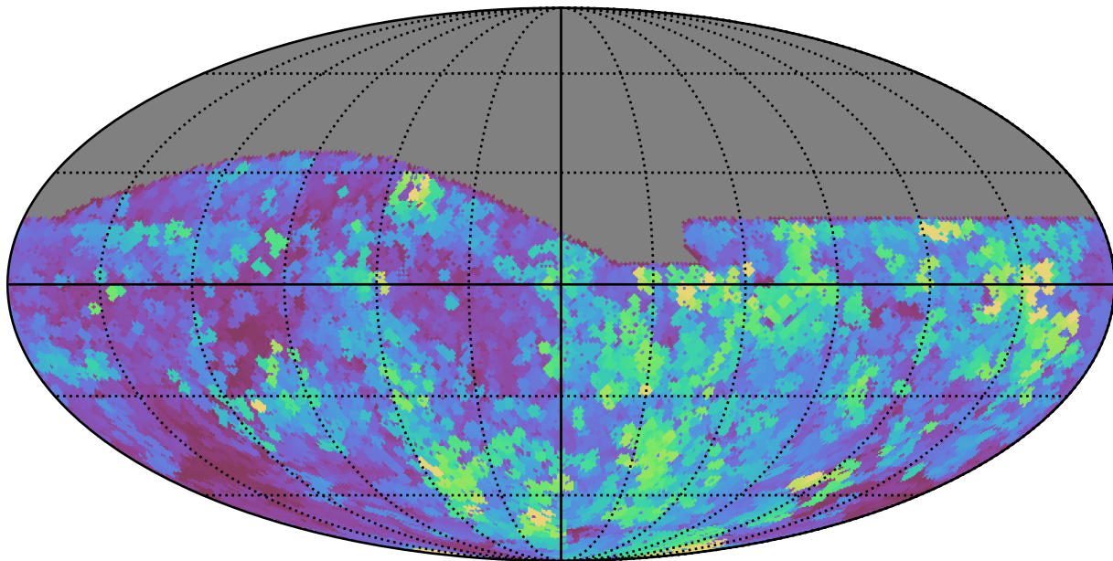
baseline_v2.0_10yrs All sky r band: Max seeingEff
