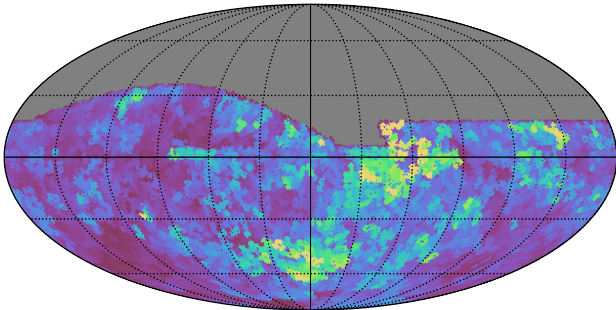
baseline_v2.0_10yrs All sky i band: Max seeingEff
