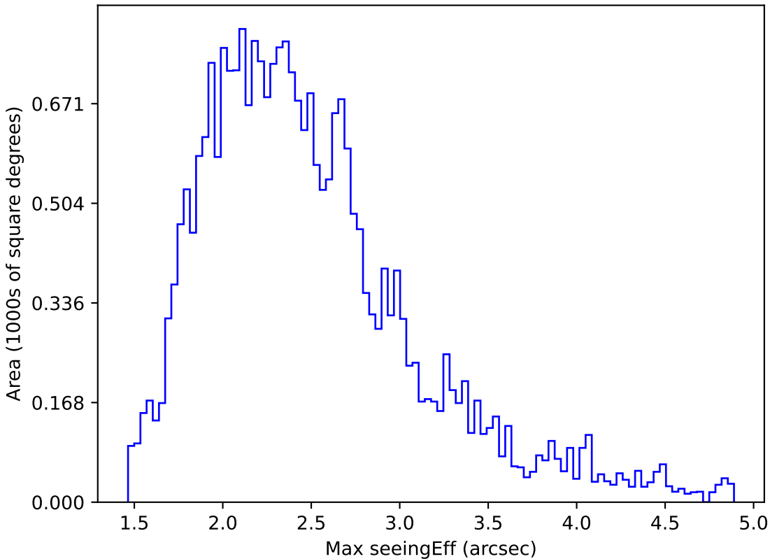
baseline_v2.0_10yrs All sky i band: Max seeingEff
