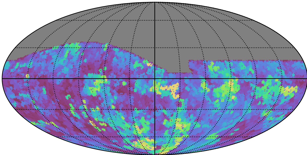
baseline_v2.0_10yrs All sky g band: Max seeingEff
