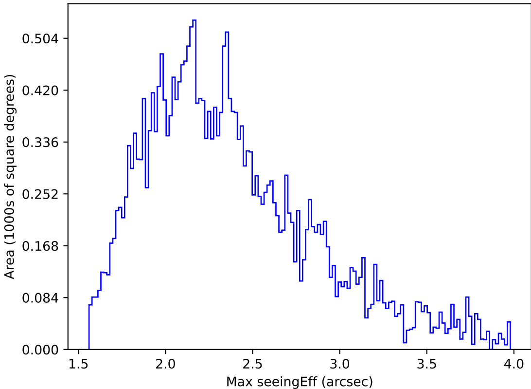
baseline_v2.0_10yrs All sky g band: Max seeingEff
