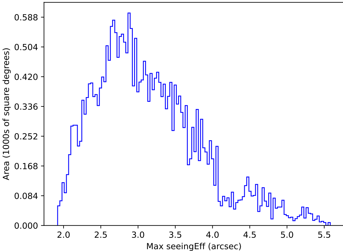
baseline_v2.0_10yrs All sky all bands: Max seeingEff
