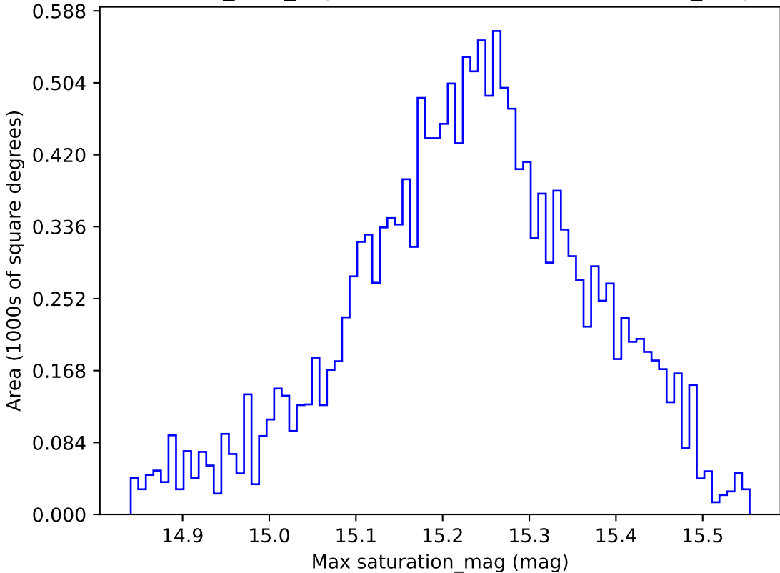
baseline_v2.0_10yrs WFD z band: Max saturation_mag
