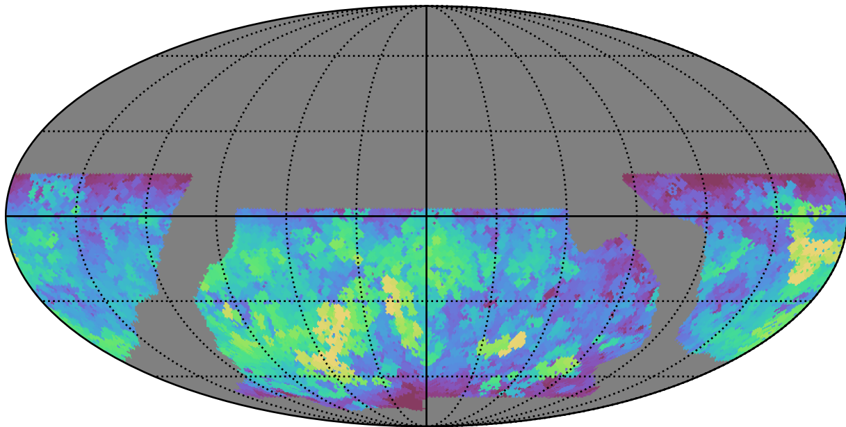
baseline_v2.0_10yrs WFD y band: Max saturation_mag
