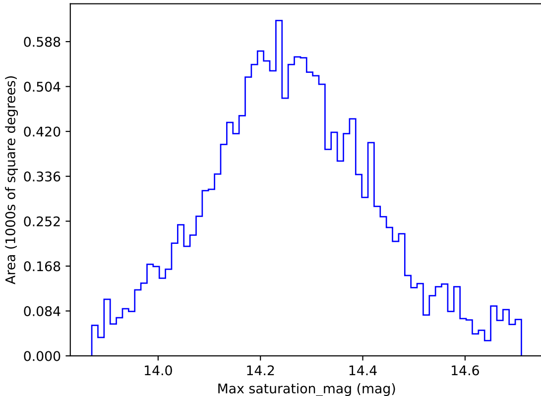
baseline_v2.0_10yrs WFD y band: Max saturation_mag
