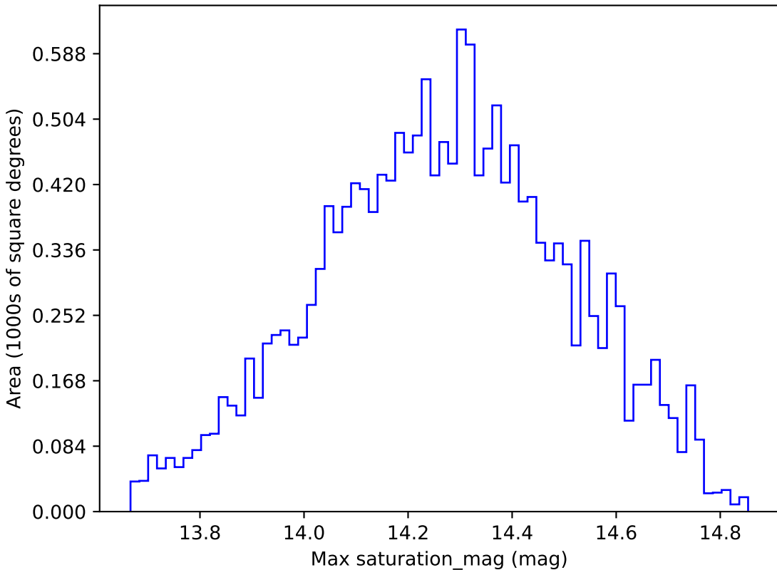
baseline_v2.0_10yrs WFD u band: Max saturation_mag
