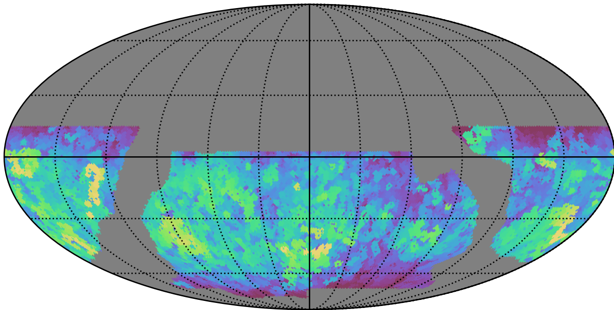
baseline_v2.0_10yrs WFD r band: Max saturation_mag
