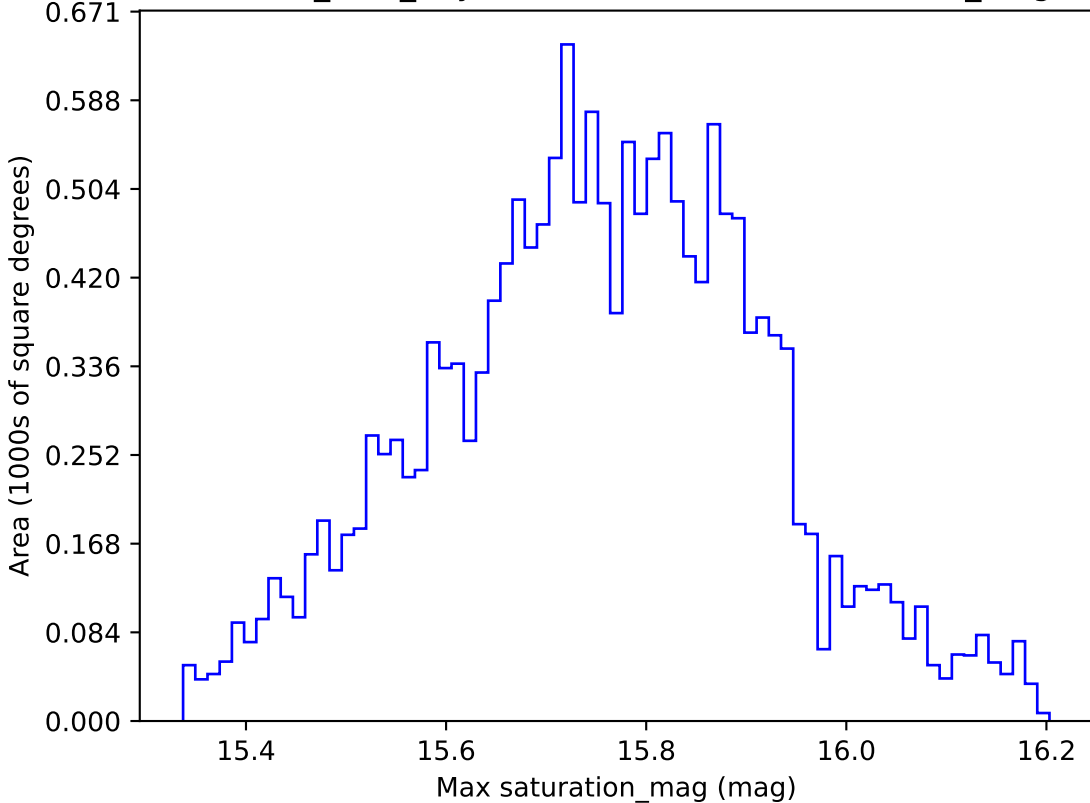
baseline_v2.0_10yrs WFD r band: Max saturation_mag
