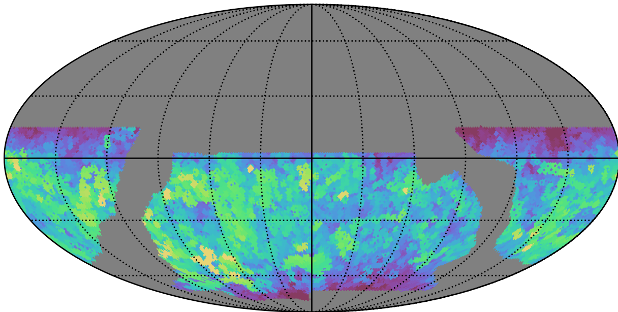
baseline_v2.0_10yrs WFD i band: Max saturation_mag
