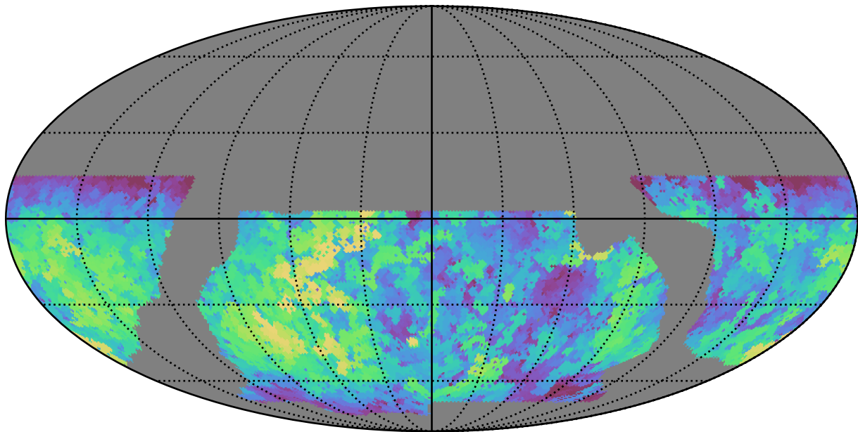
baseline_v2.0_10yrs WFD g band: Max saturation_mag
