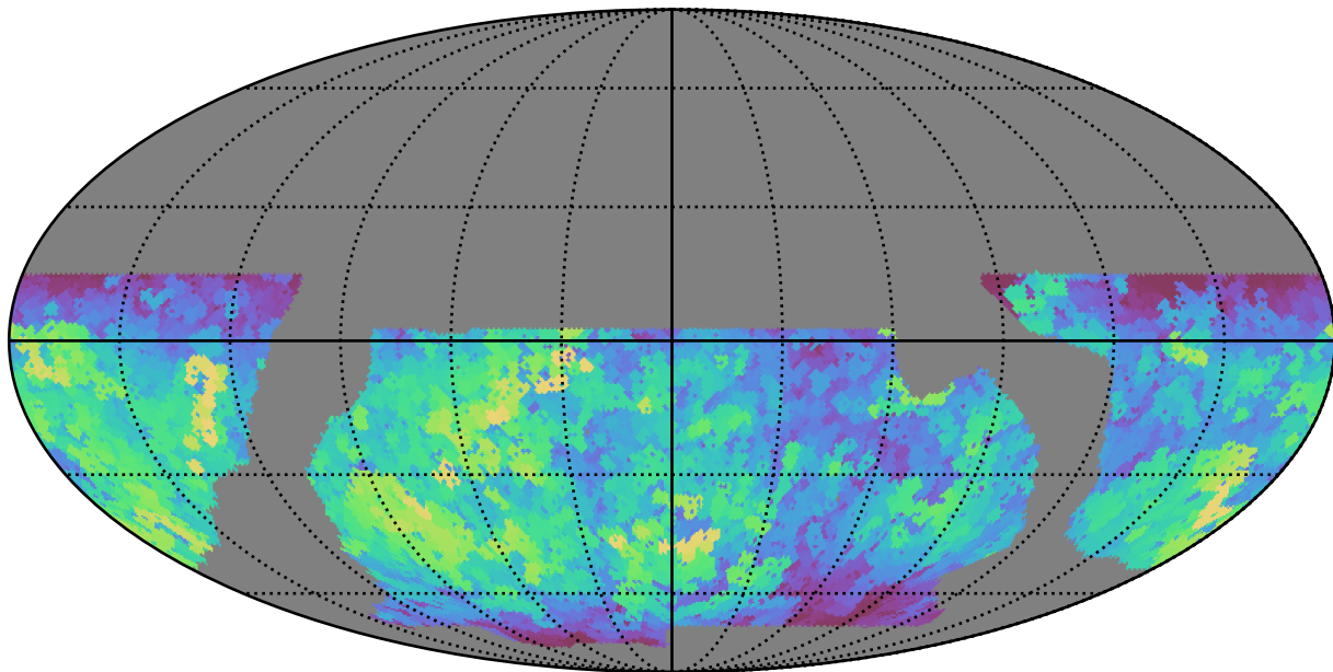
baseline_v2.0_10yrs WFD all bands: Max saturation_mag
