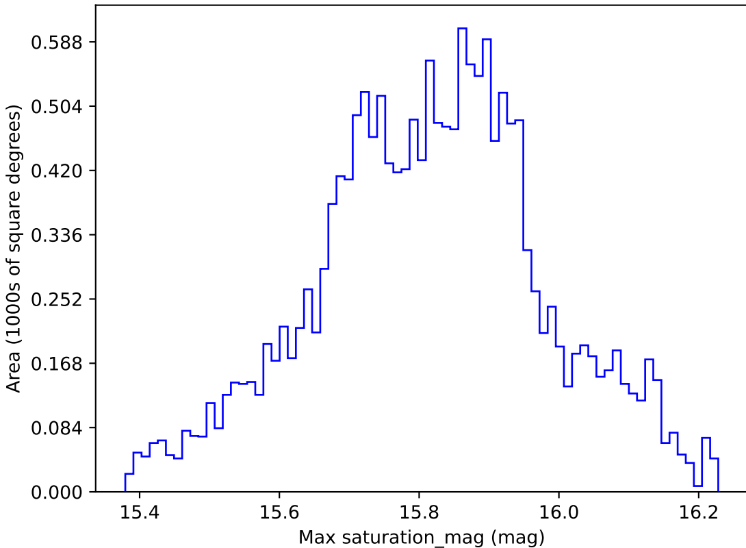
baseline_v2.0_10yrs WFD all bands: Max saturation_mag
