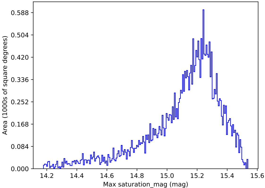
baseline_v2.0_10yrs All sky z band: Max saturation_mag
