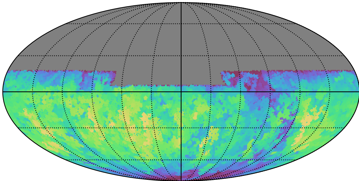
baseline_v2.0_10yrs All sky u band: Max saturation_mag
