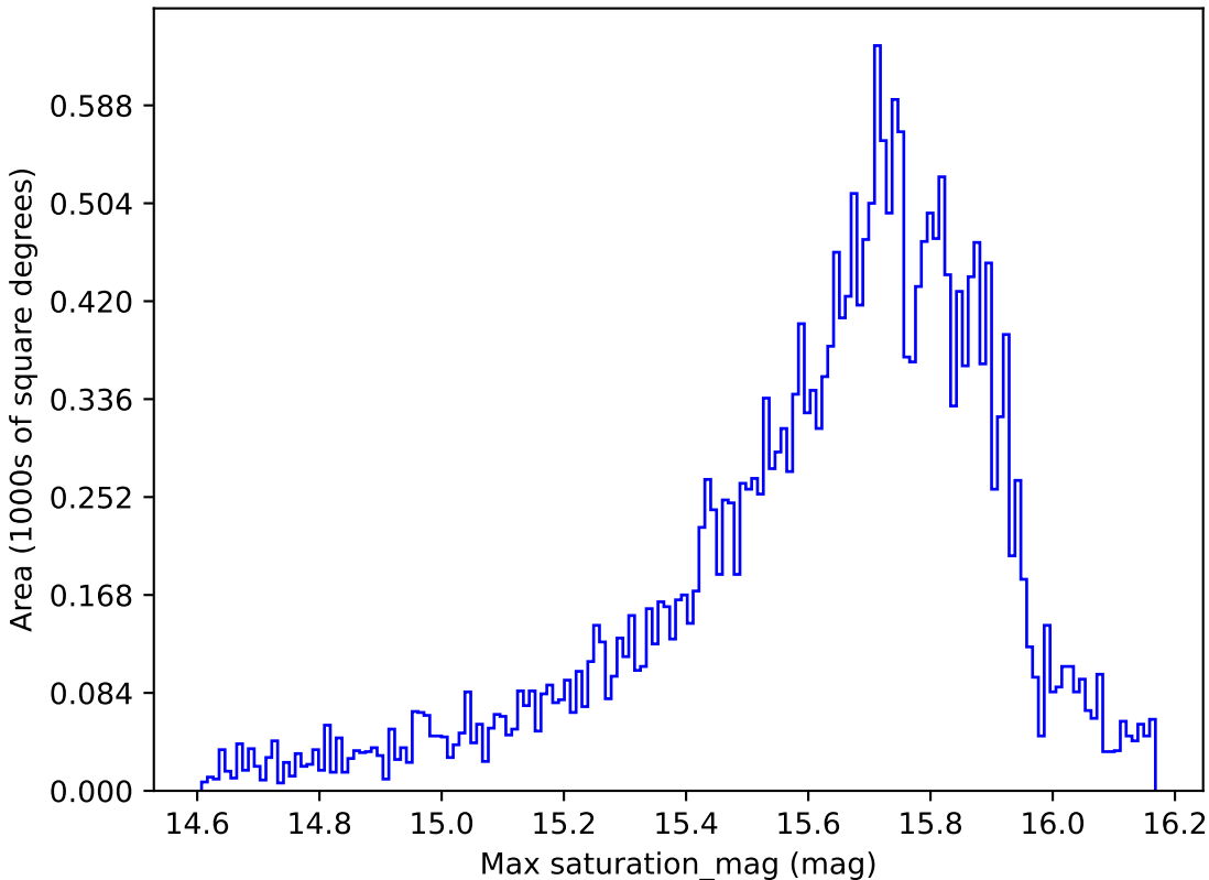
baseline_v2.0_10yrs All sky r band: Max saturation_mag
