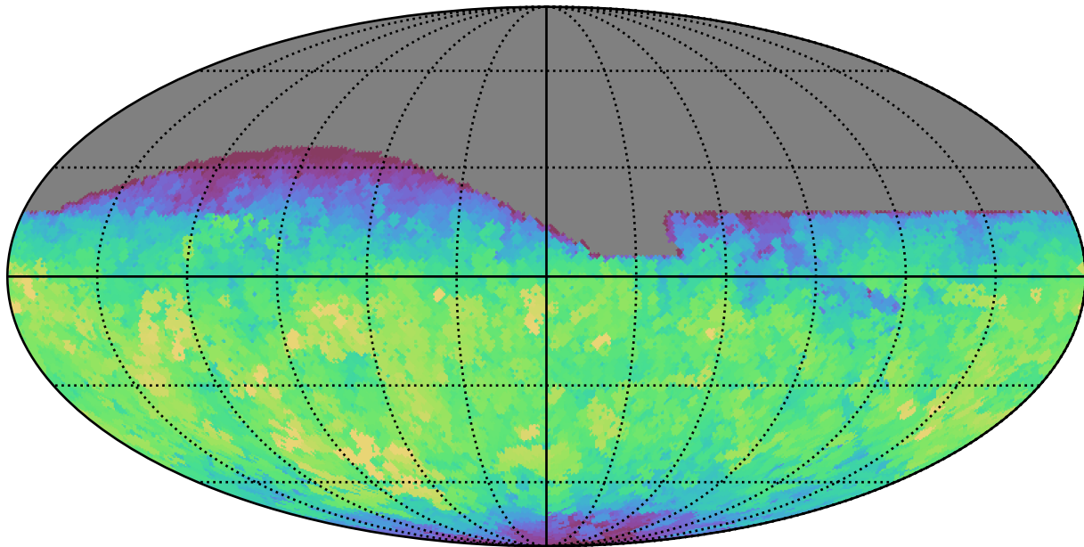
baseline_v2.0_10yrs All sky i band: Max saturation_mag
