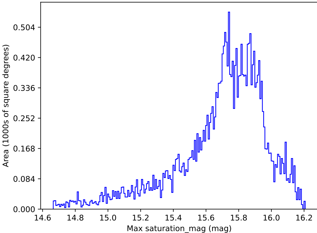
baseline_v2.0_10yrs All sky all bands: Max saturation_mag
