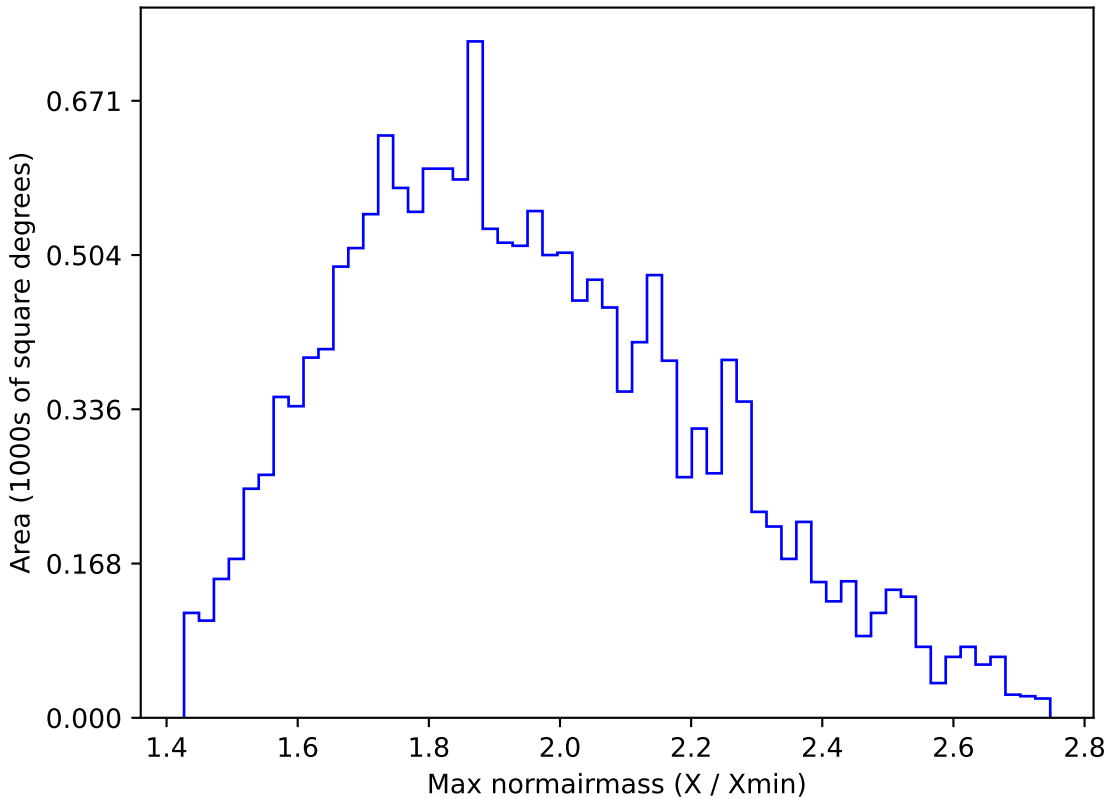
baseline_v2.0_10yrs WFD z band: Max normairmass
