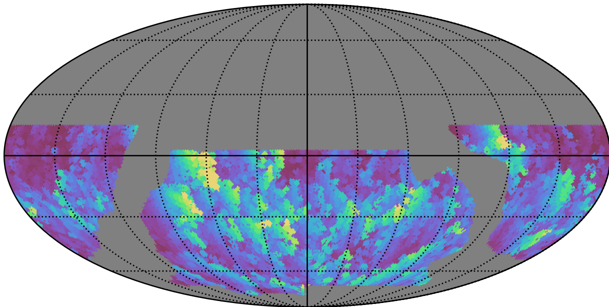
baseline_v2.0_10yrs WFD u band: Max normairmass
