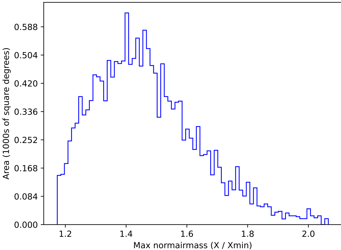
baseline_v2.0_10yrs WFD u band: Max normairmass
