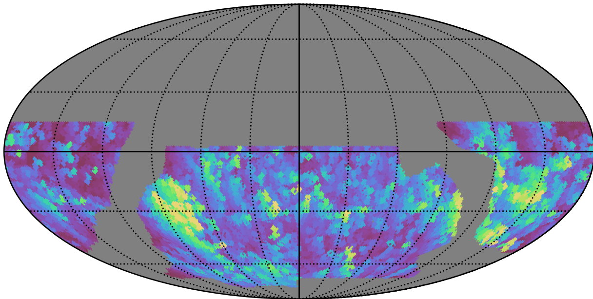
baseline_v2.0_10yrs WFD i band: Max normairmass
