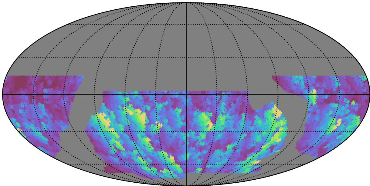
baseline_v2.0_10yrs WFD g band: Max normairmass
