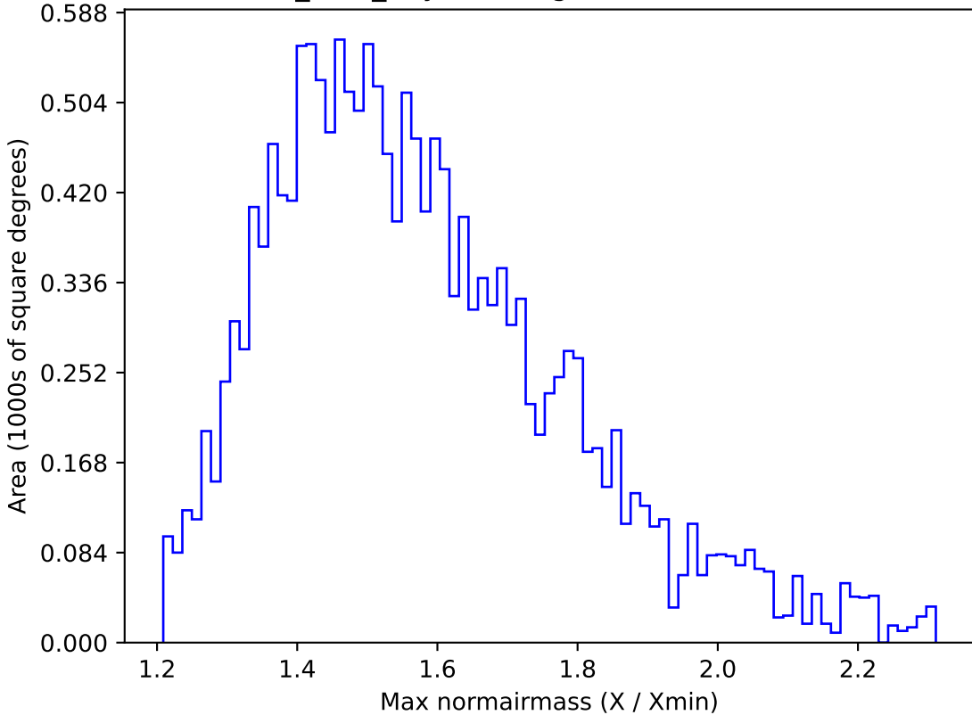
baseline_v2.0_10yrs WFD g band: Max normairmass
