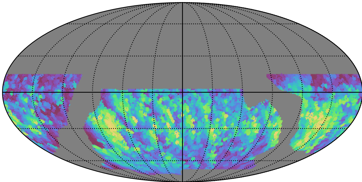
baseline_v2.0_10yrs WFD all bands: Max normairmass
