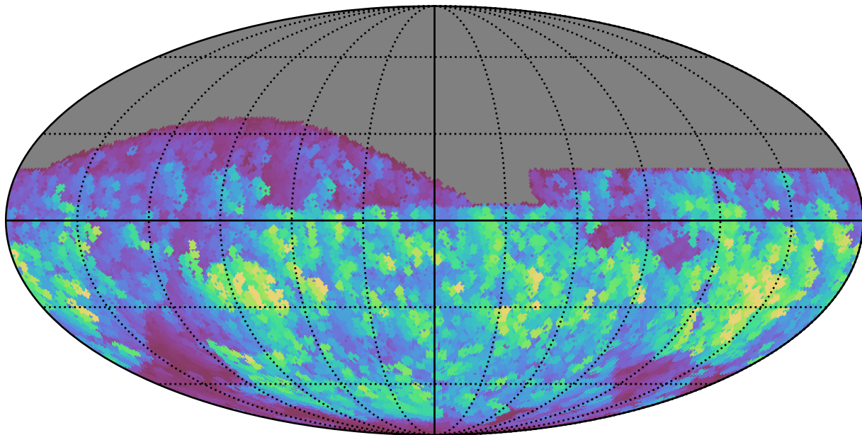
baseline_v2.0_10yrs All sky z band: Max normairmass
