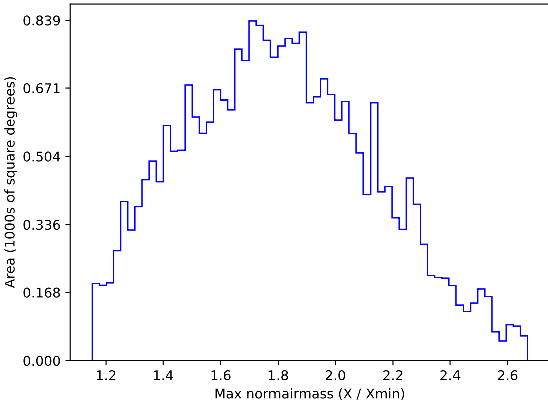
baseline_v2.0_10yrs All sky z band: Max normairmass
