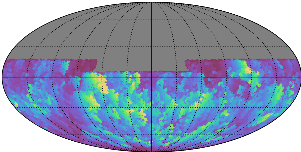
baseline_v2.0_10yrs All sky u band: Max normairmass
