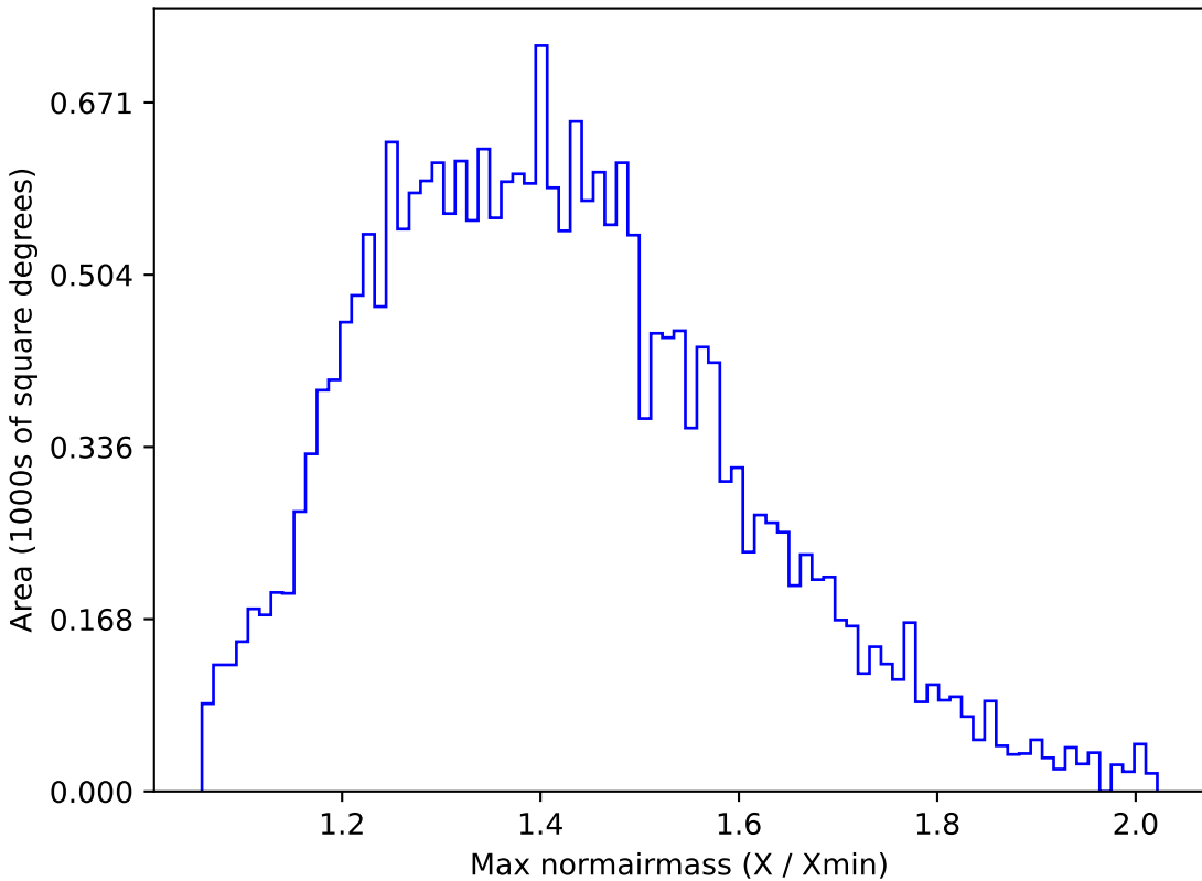
baseline_v2.0_10yrs All sky u band: Max normairmass
