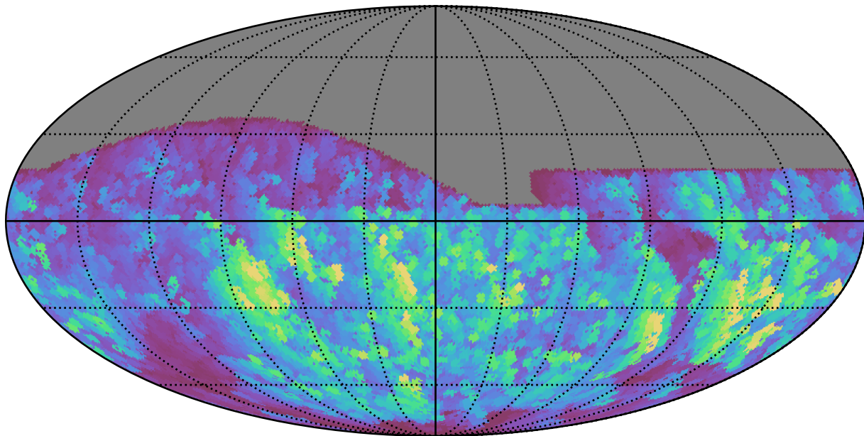
baseline_v2.0_10yrs All sky r band: Max normairmass
