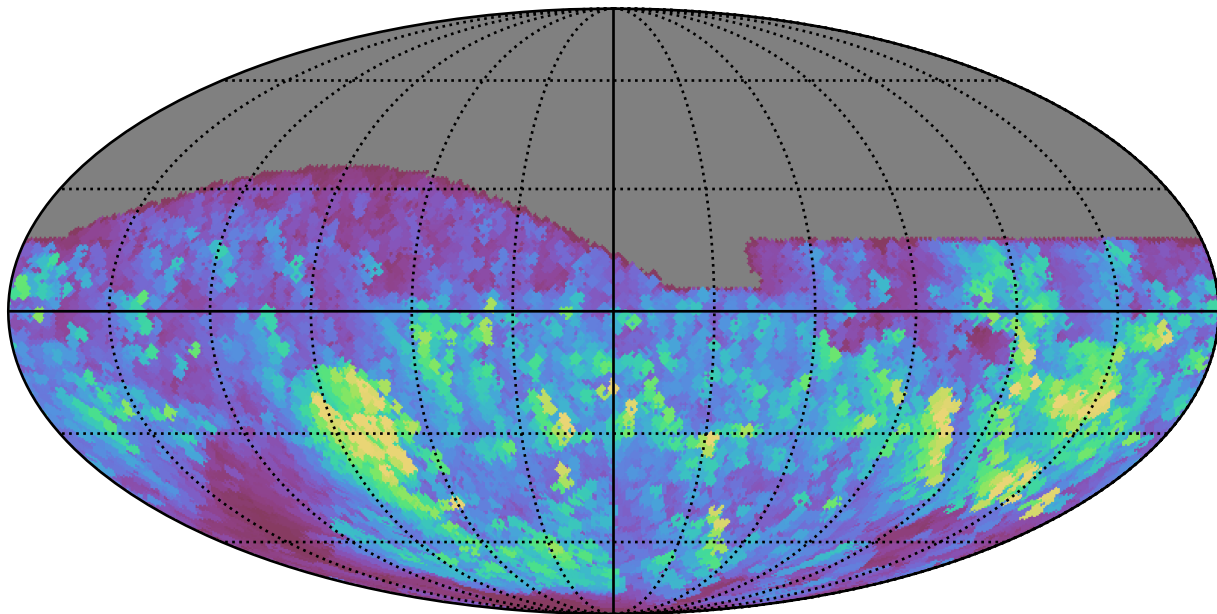
baseline_v2.0_10yrs All sky i band: Max normairmass
